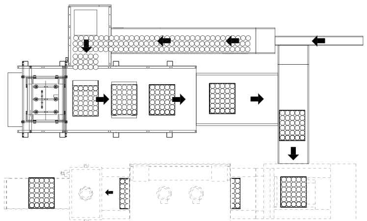
Example of Complete System CUH Tray Packer and SLU Shrink Wrapper
